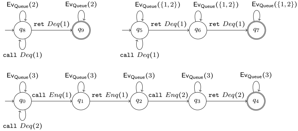
Figure 2: A non-deterministic automaton recognizing R_{EnqDeq} violations. The top-left branch recognizes executions which have a Deq with no corresponding Enq . The top-right branch recognizes two Deq 's returning the same value, which is not supposed to happen in a differentiated execution. The bottom branch recognizes FIFO violations. By the closure properties of implementations, we can assume the \text{call } Deq(2) are at the beginning.
