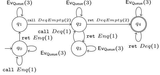
Figure 4: An automaton recognizing R_{DeqEmpty} violations, for which the queue is non-empty, with data value 1, for the span of DeqEmpty . We assume all call\ Enq(1) actions occur initially without loss of generality due to implementations' closure properties.
