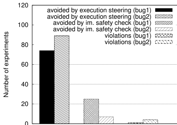
Figure 9: In 200 runs that expose Paxos safety violations due to two injected errors, CrystalBall successfully avoided the inconsistencies in all but 1 and 4 cases, respectively.
