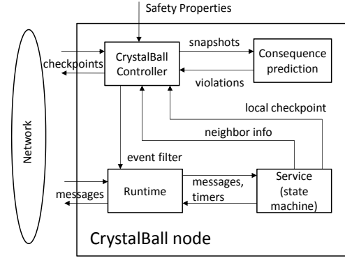
Figure 4: High-level overview of CrystalBall
