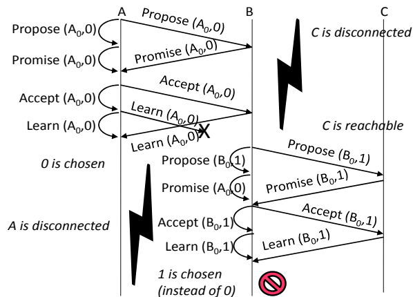
Figure 8: Scenario that exposes a previously reported Paxos violation of a safety property (two different values are chosen in the same instance).
