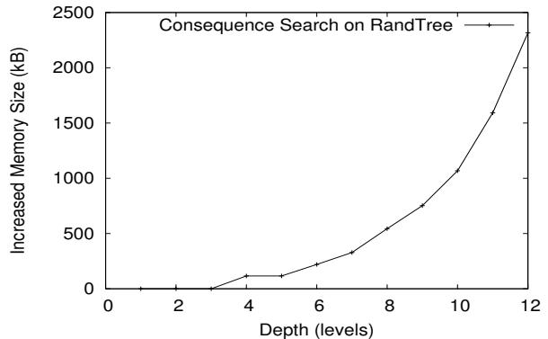
Figure 10: The memory consumed by consequence prediction (RandTree, depths 7 to 8) fits in an L2 CPU cache.
