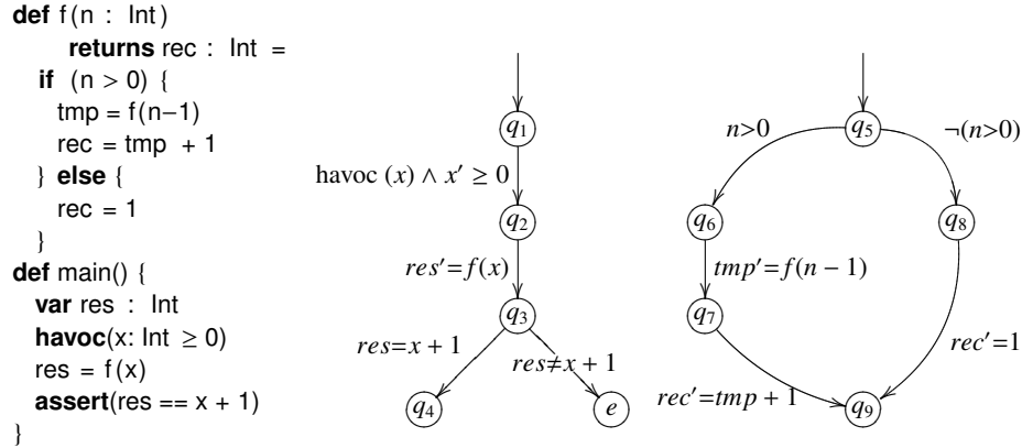
Fig. 1. A recursive program and its control flow graph (see Sect. 3).
